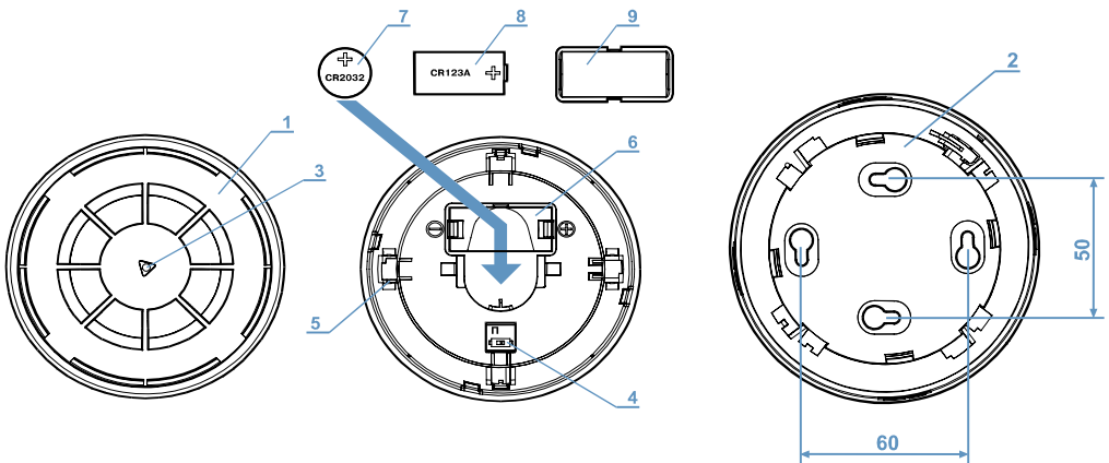
Figure 2 - SG-XXX detector
