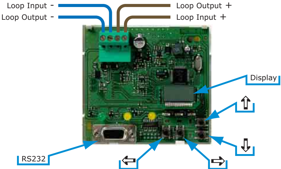
Figure 1 - Board and terminals
