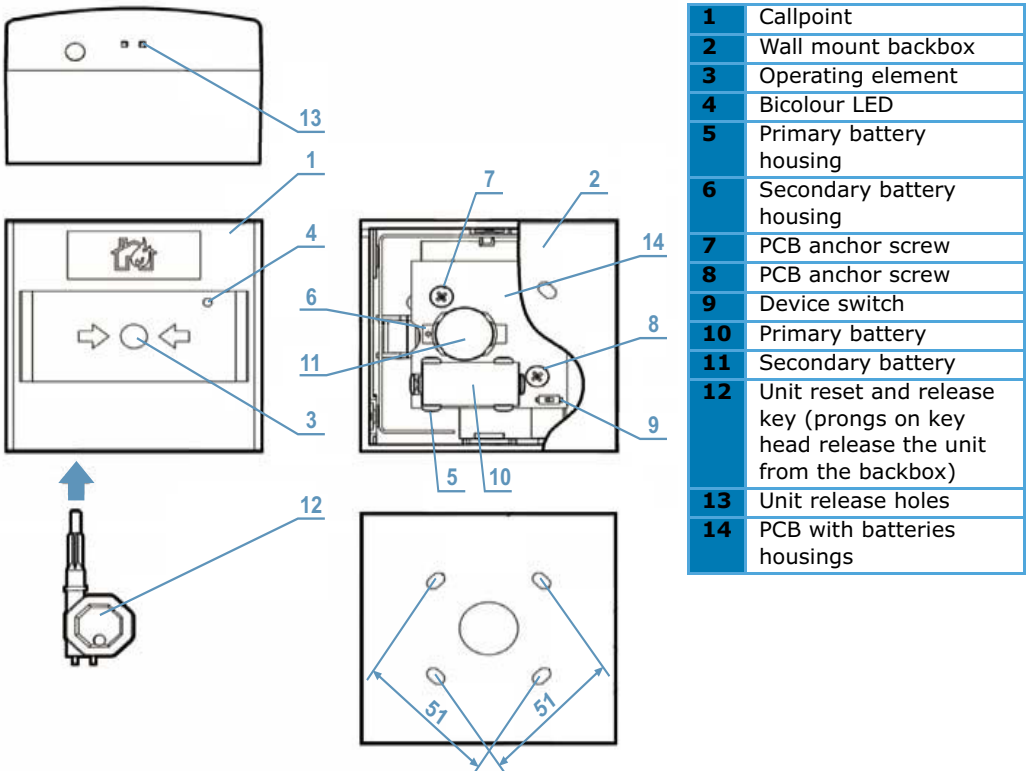
Figure 5 - Manual resettable callpoint
