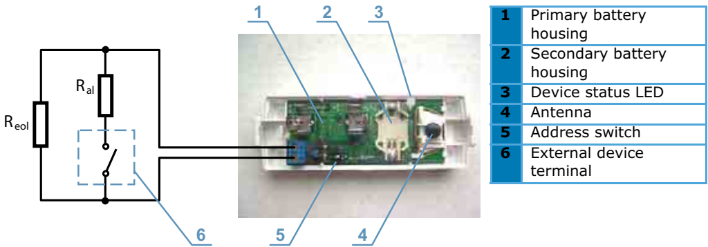
Figure 7 - Terminals
