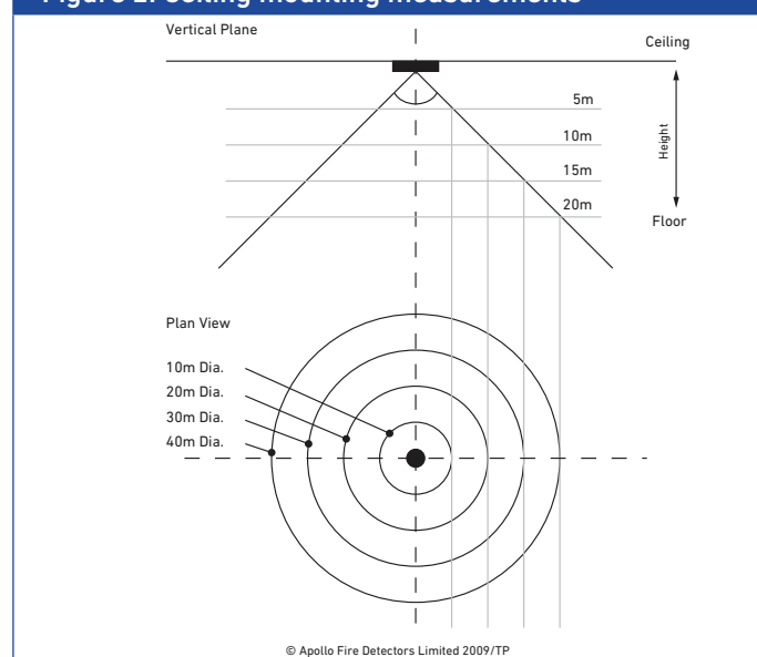
Figure 2: Ceiling mounting measurements
