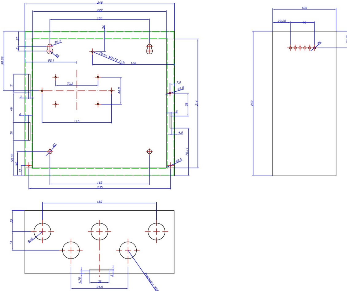
Figure 3: Door and main box measurements (mm).
