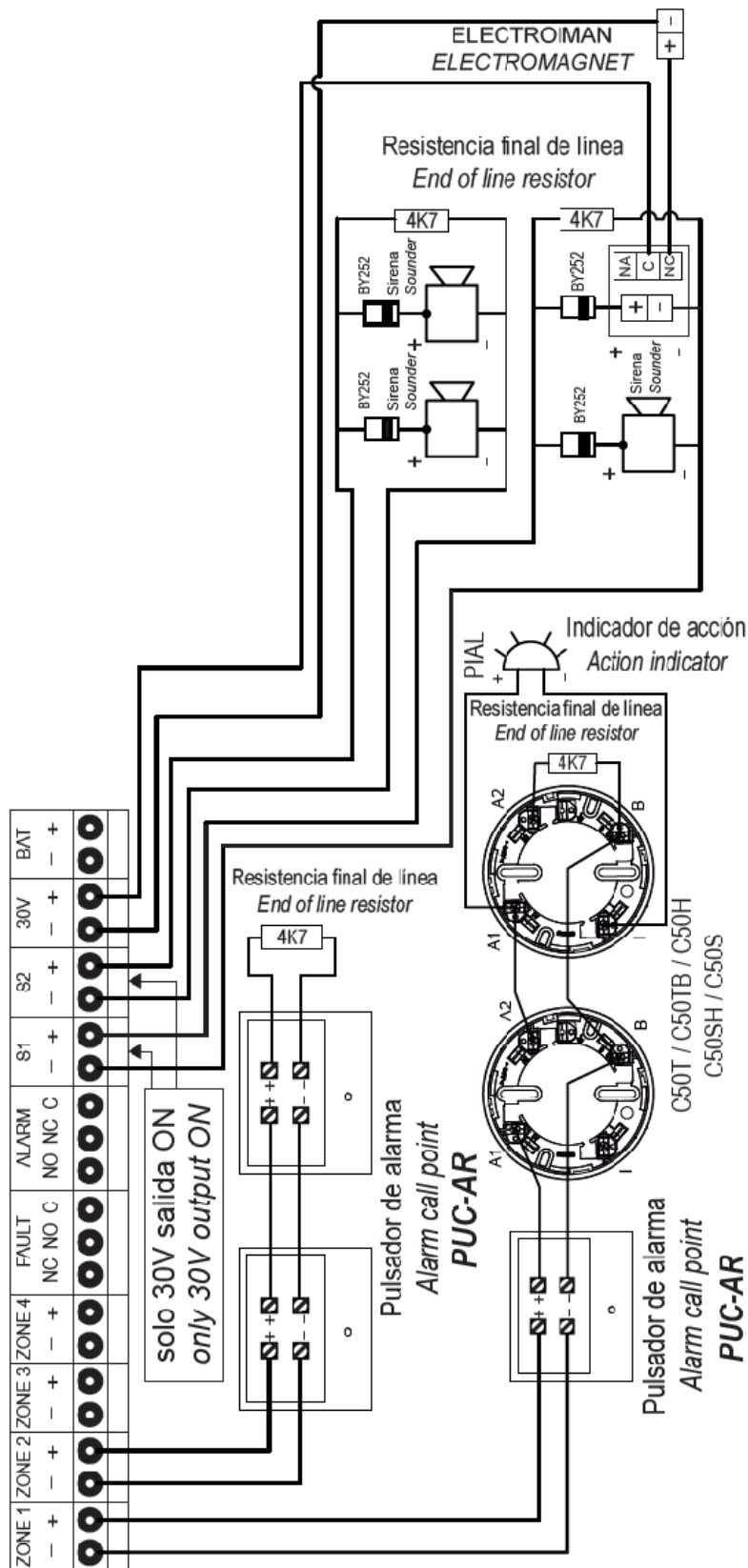
Figure 6: Example of IRON02/04 general wiring diagram
