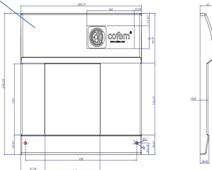
Figure 2: Diagram of box and main door
