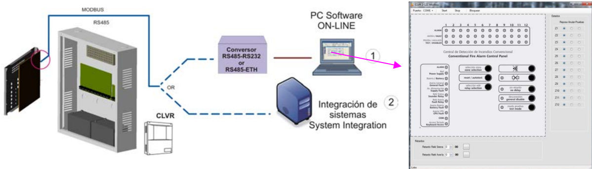
Figura 13 MODBUS Communication
