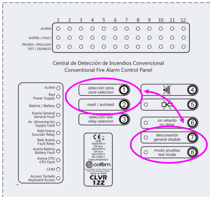
Figure 7: Keys used in the control panel access levels CLVR02Z / 04Z / 08Z / 12Z
