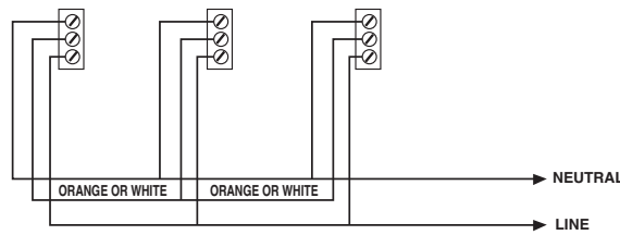
FOR INTERCONNECTING: USE A MINIMUM OF 1.5mm 2 CABLE
