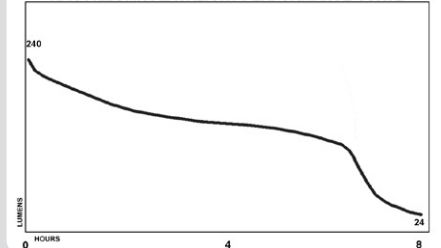
XPR-5522GMX FLASHLIGHT PERFORMANCE CURVE
