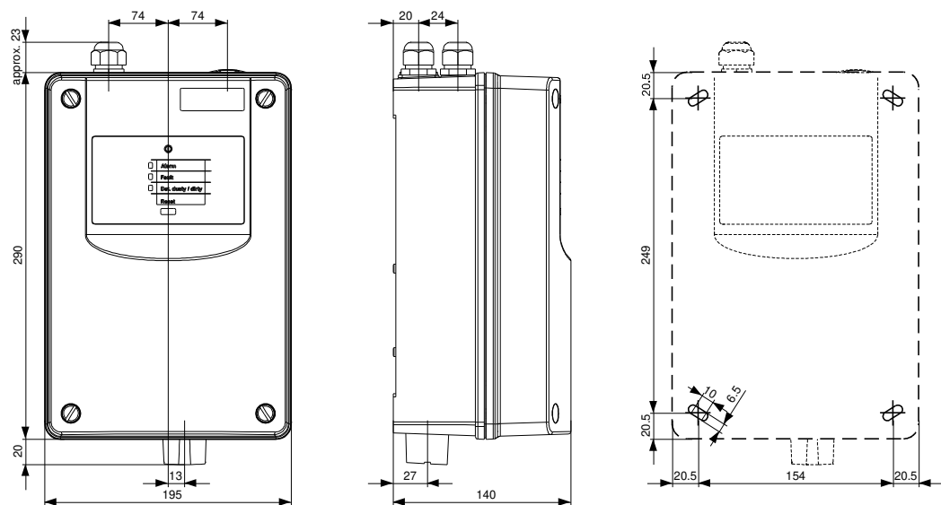
Figure 4. Detector housing dimensioned drawing
