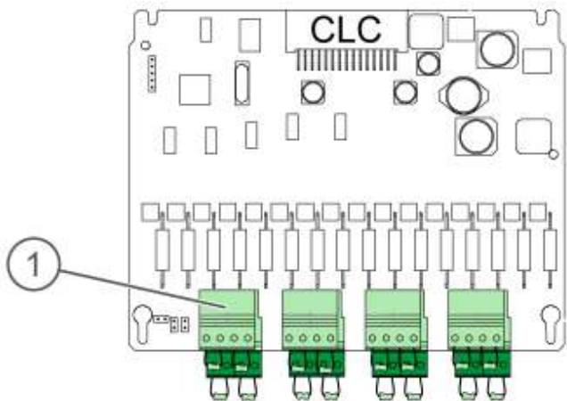
Figure 6. Terminals on the CLC circuit board
