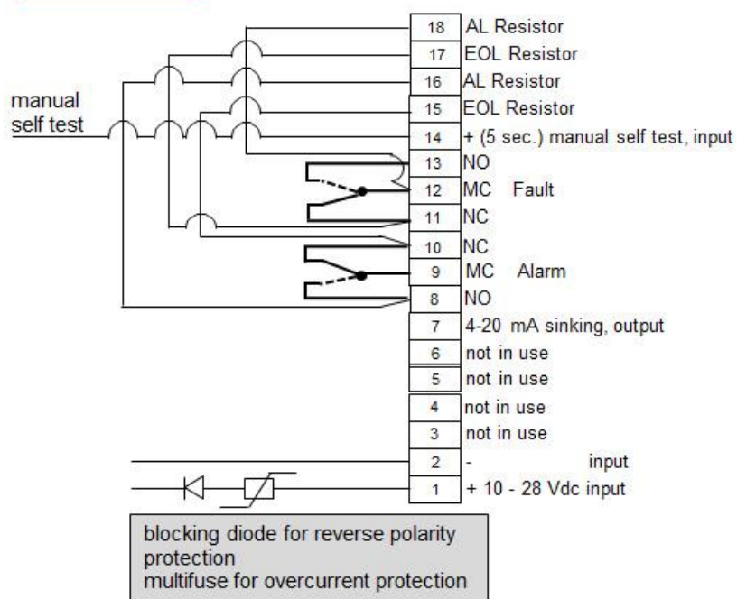
Connection diagram
