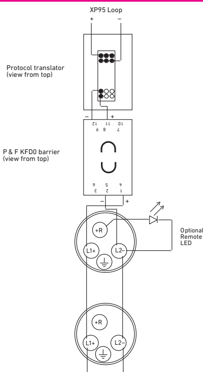
Figure 3: Detail of wiring diagram for XP95 I.S. Zone
