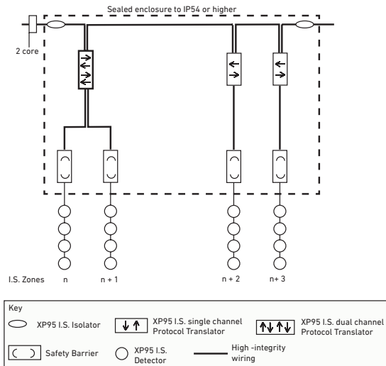
Figure 2: Schematic wiring diagram of XP95 I.S. circuit using a dual channel protocol translator
