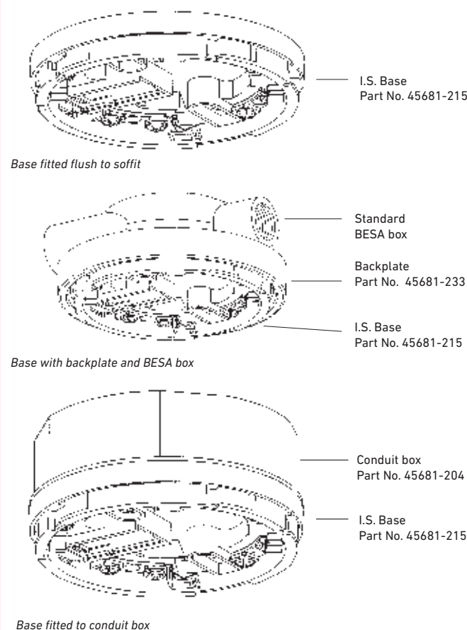
Figure 4: Permissible methods of mounting I.S. detector bases
