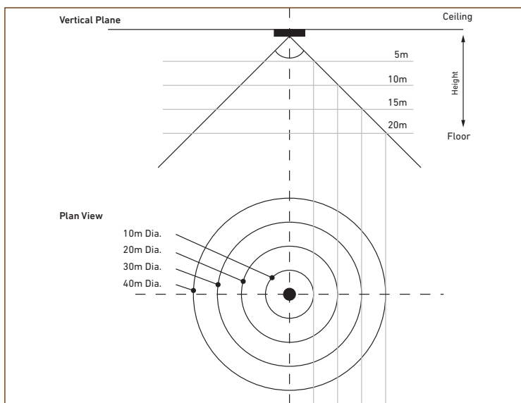
Figure 2: Ceiling mounting measurements
