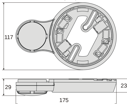
DBS720
